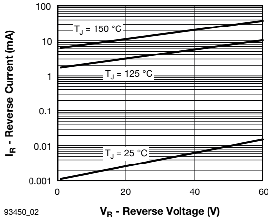
93450_02 V R - Reverse Voltage (V) Fig. 2 - Typical Values of Reverse Current vs. Reverse Voltage
