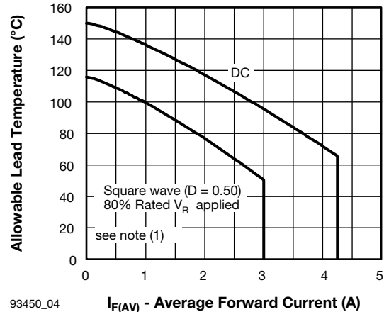
93450_04 I F(AV) - Average Forward Current (A) Fig. 4 - Maximum Allowable Lead Temperature vs. Average Forward Current
