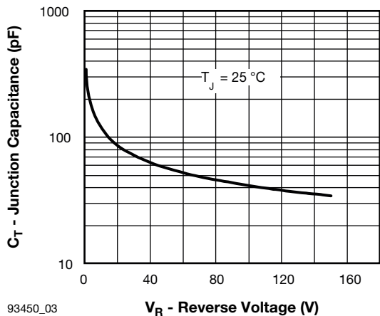
93450_03 V R - Reverse Voltage (V) Fig. 3 - Typical Junction Capacitance vs. Reverse Voltage
