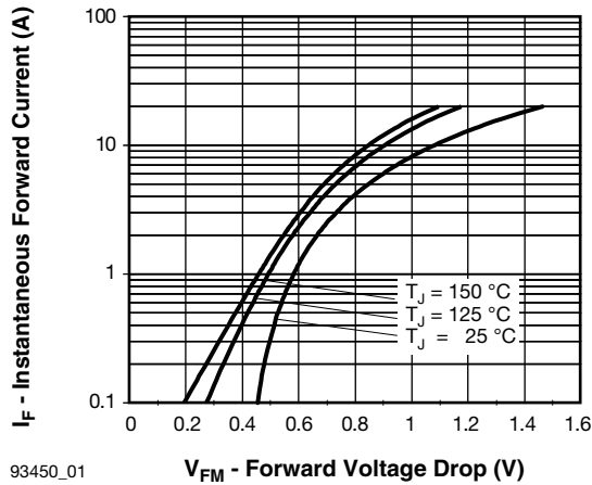
93450_01 V FM - Forward Voltage Drop (V) Fig. 1 - Maximum Forward Voltage Drop Characteristics
