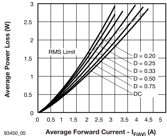
93450_05 Average Forward Current - I F(AV) (A) Fig. 5 - Forward Power Loss Characteristics
