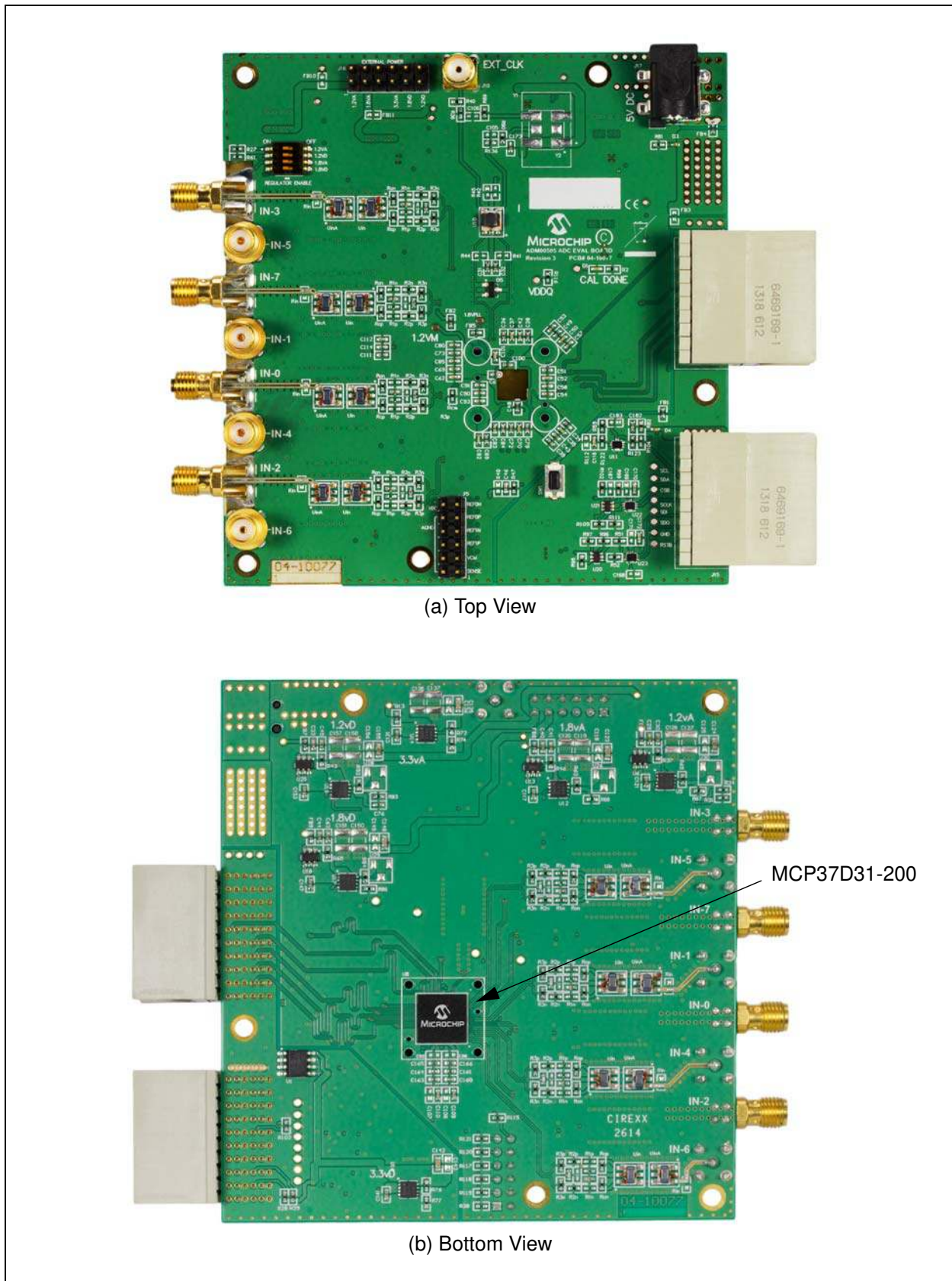
FIGURE 1-2: MCP37X3X-200 16-Bit 200 Mps ADC VTLA Evaluation Board (ADM00505).
