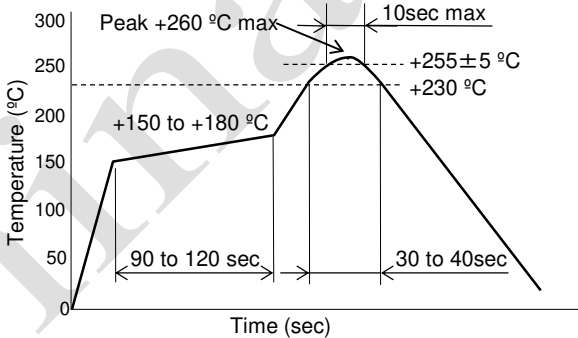
Fig.5 Reflow profile (Lead Free Available)
