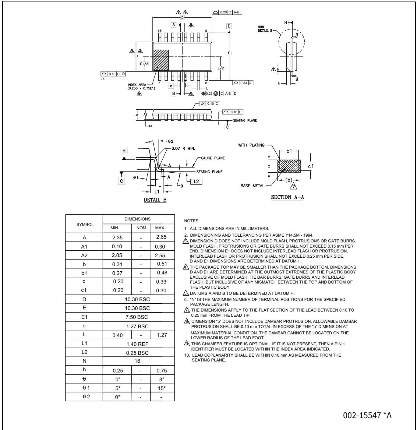
Figure 150 SOIC 16-lead, 300-mil body width (SO3016)
