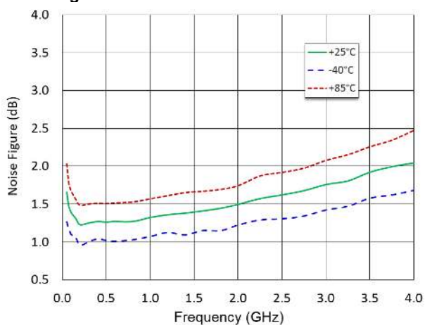
Noise Figure
