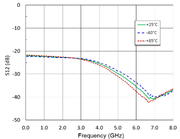
Reverse Isolation
