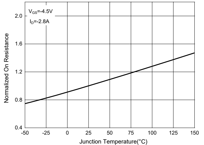
Fig.4-NormalizedOnResistanceCharacteristics
