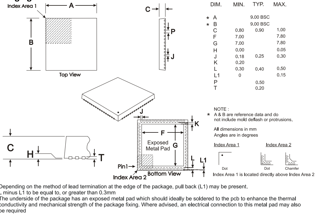
Figure 28 Mechanical Outline of 64-pin VQFN (Q1)
