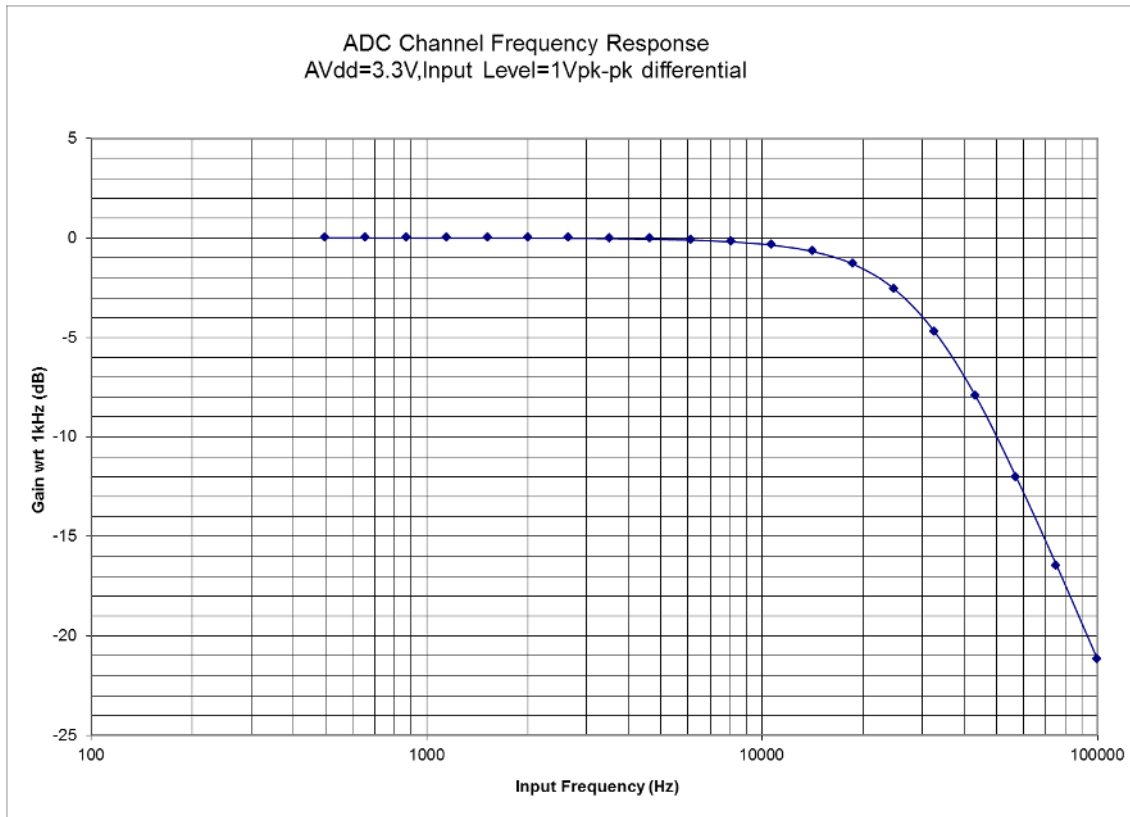
Figure 13 ADC Channel Frequency Response
