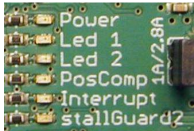
Figure 5: TMCM-1110 StepRocker LEDs
