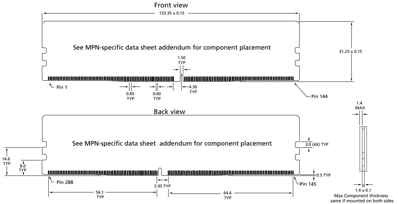
Figure 1: 288-Pin DDR4 RDIMM
