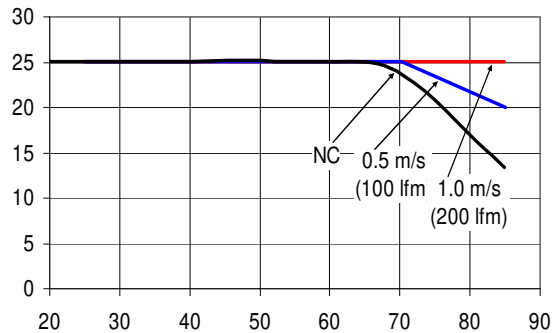
Figure 15. Thermal Derating Curves for the QPW025A0F41 module at 48Vin. Airflow is in the transverse direction (Vin- to Vin+).
