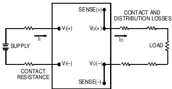
Figure 9. Output Voltage and Efficiency Test Setup.
