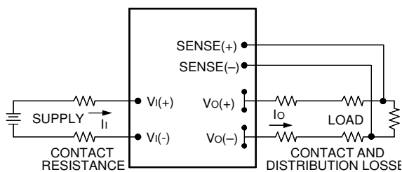
Figure 11. Circuit Configuration to program output voltage using external resistor.
