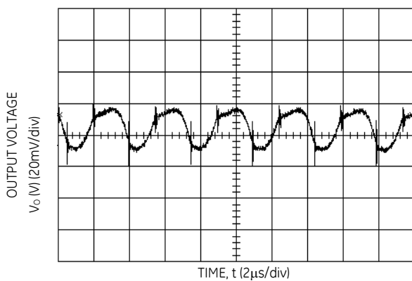
Figure 3. Typical Output Ripple and Noise at V_{in} = 48Vdc .
