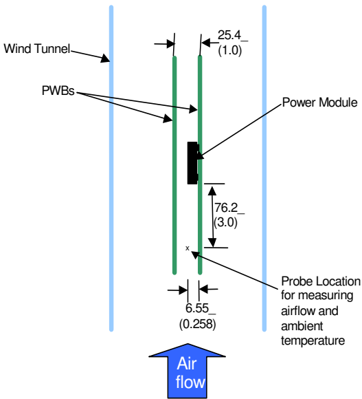
Figure 13. Thermal Test Set up.
