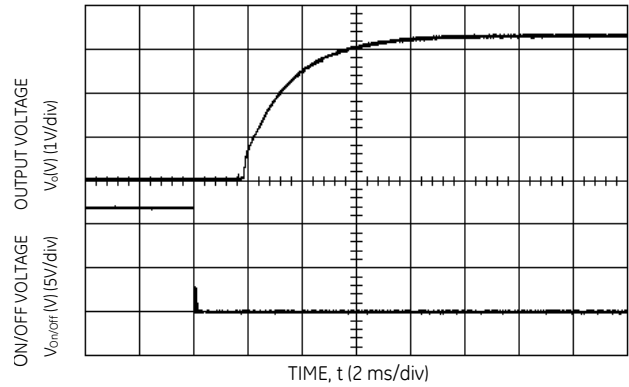
Figure 4. Typical Start-Up Characteristics from Remote ON/OFF.
