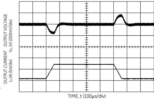
Figure 5. Transient Response to Dynamic Load Change from 50% to 25% to 50% of full load current.
