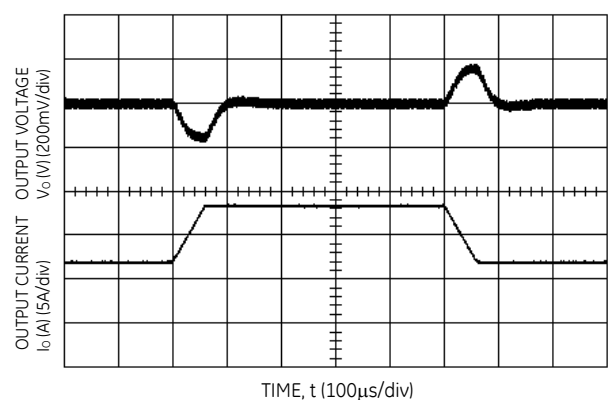
Figure 6. Transient Response to Dynamic Load Change from 75% to 50% to 75% of full load current.
