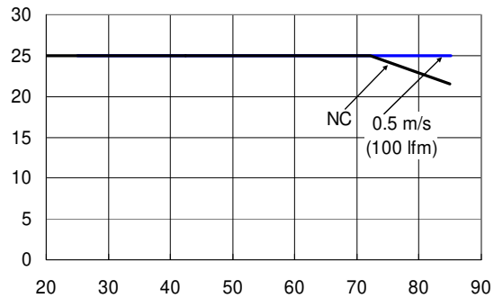
Figure 16. Thermal Derating Curves for the QPW025A0F41-H baseplate module at 48Vin. Airflow is in the transverse direction (Vin- to Vin+).
