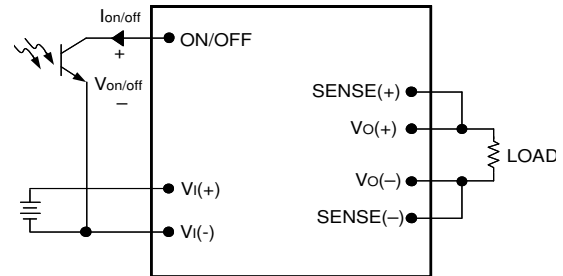
Figure 10. Circuit configuration for using Remote On/Off Implementation.
