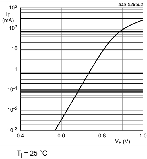
Fig. 3. Forward current as a function of forward voltage; typical values (BZX884S-B/C7V5-Q)
