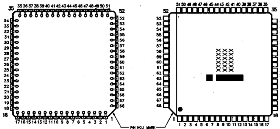
Figure 2. 80C186 Pinout Diagrams
