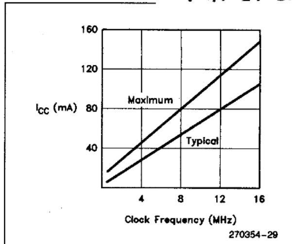
Figure 46. I CC vs Frequency
