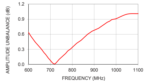
TCN3-11+ AMPLITUDE UNBALANCE
