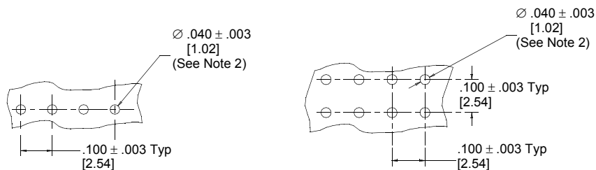
Recommended Mounting Hole Pattern
