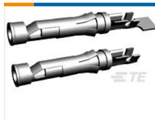
TE Part #66399-3 III+ SKT,24-20,15AU/FL,LP
