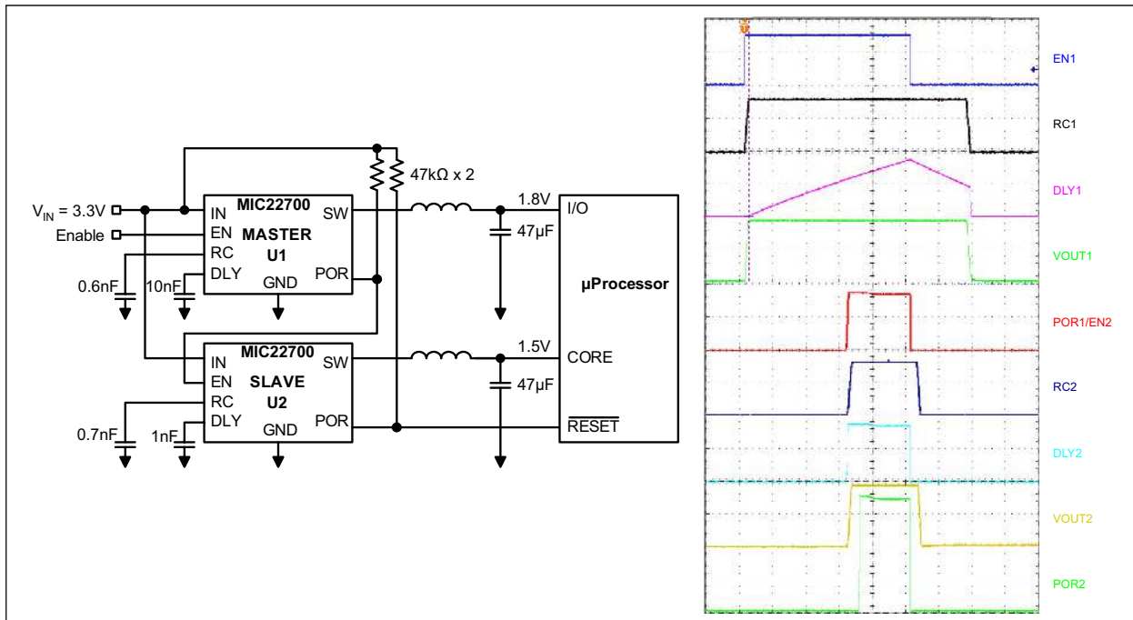
FIGURE 2-26: Sequencing Circuit and Waveform.
