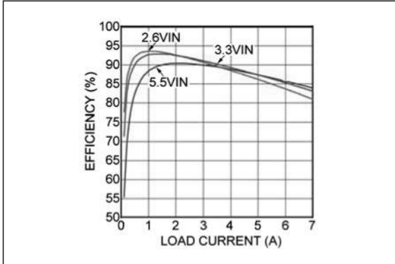
FIGURE 2-13: Efficiency at 1.8V_{OUT} .
