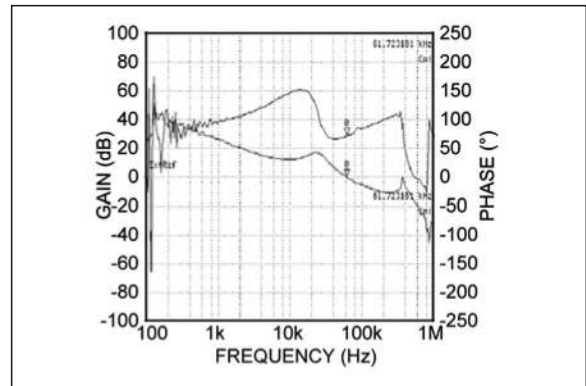
FIGURE 2-17: Bode Plot ( V_{IN} = 5.0V , V_{OUT} = 3.3V ).
