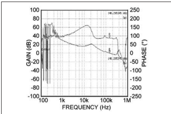
FIGURE 2-15: Bode Plot ( V_{IN} = 3.6V , V_{OUT} = 1.8V ).
