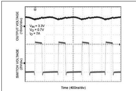
FIGURE 2-21: Switching Waveforms.
