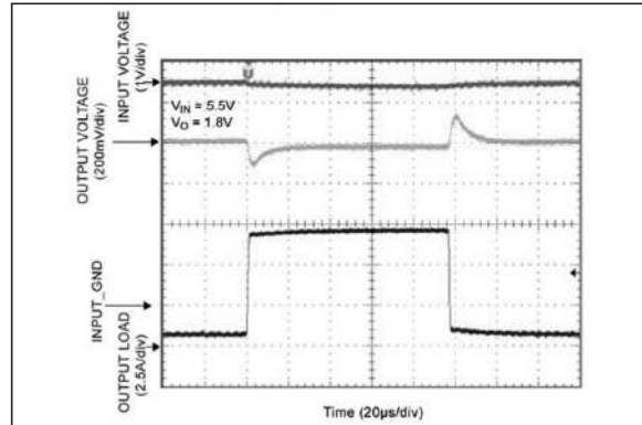
FIGURE 2-22: Transient Response.
