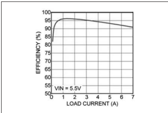
FIGURE 2-14: Efficiency at 3.3V_{OUT} .
