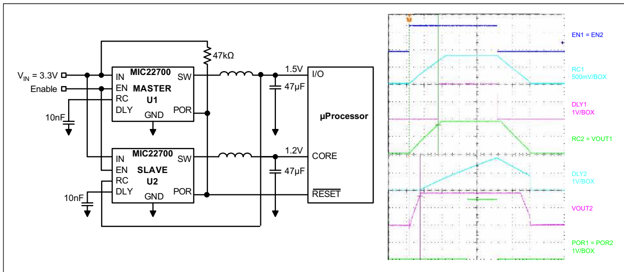
FIGURE 2-27: Tracking Circuit and Waveform.
