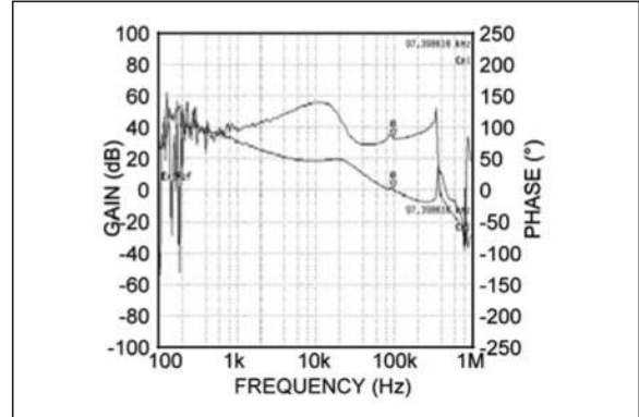
FIGURE 2-16: Bode Plot ( V_{IN} = 5.5V , V_{OUT} = 1.8V ).
