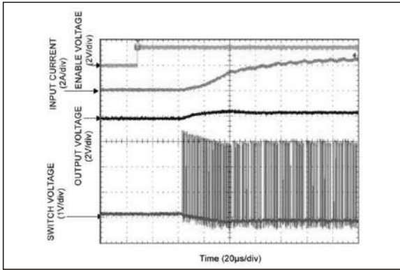
FIGURE 2-25: Start-Up into Short-Circuit.
