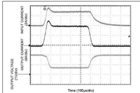
FIGURE 2-24: Current Limit Behavior.
