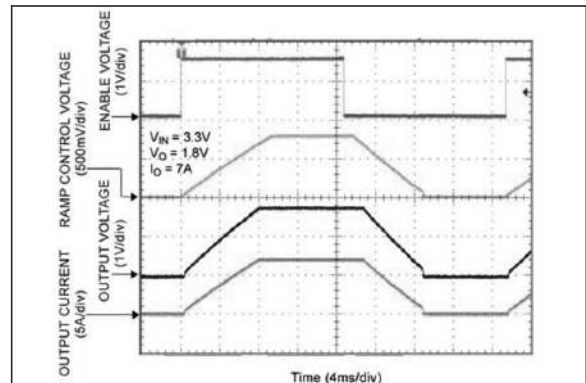
FIGURE 2-18: Start-Up/Shutdown ( C_{RC} = 10\text{ nF} ).
