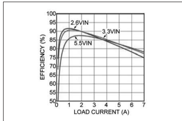
FIGURE 2-12: Efficiency at 1.2V_{OUT} .
