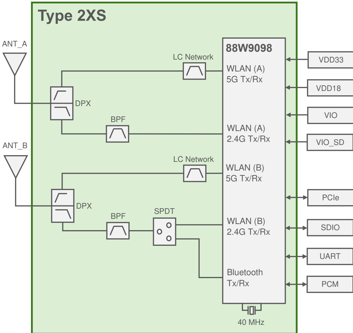
Figure 1: Block Diagram
