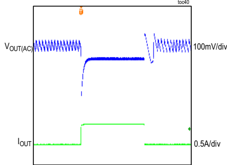
MAX17630A LOAD TRANSIENT BETWEEN 20mA AND 0.5A FIGURE 3 CIRCUIT
