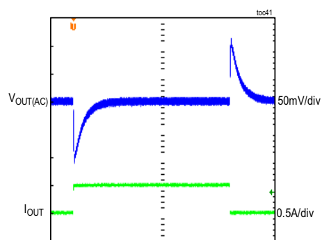
MAX17630B LOAD TRANSIENT BETWEEN 0A AND 0.5A FIGURE 4 CIRCUIT
