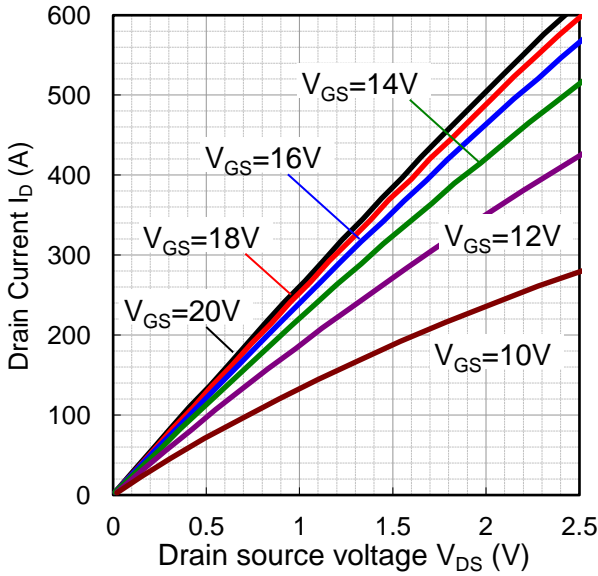
Fig.1 Output characteristic 25°C (TYP)
