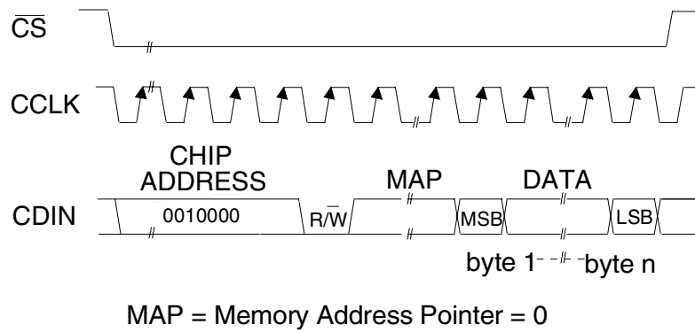
Figure 7. Control Port Timing, SPI mode
