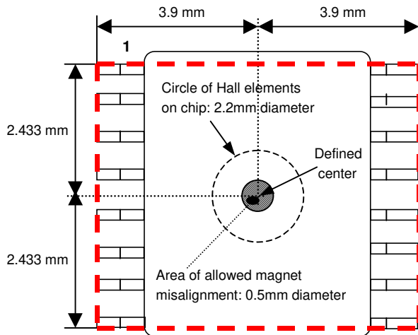
Figure 4: Tolerances of magnet placement
