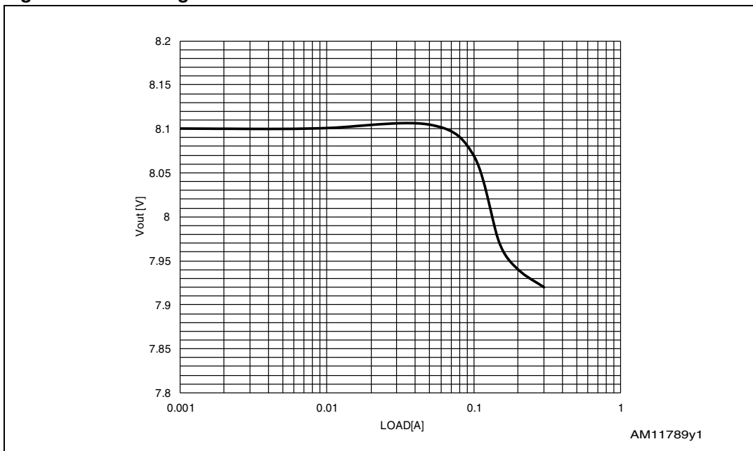
Figure 30. Load regulation
