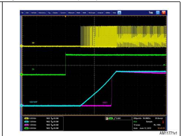
Figure 11. Power-up sequence, 69 Ω load
