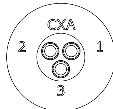
WIRE VIEW 4182-3SG-300
