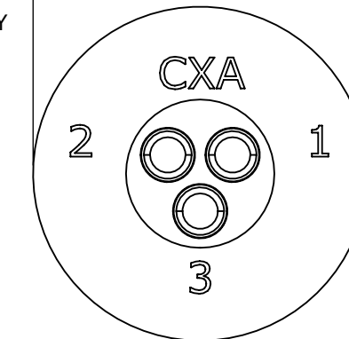
WIRE VIEW P/N: 4182-3SG-300
