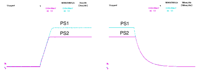
Figure 40: Sequential Start-up
