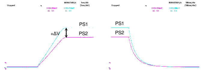
Figure 41: Simultaneous
