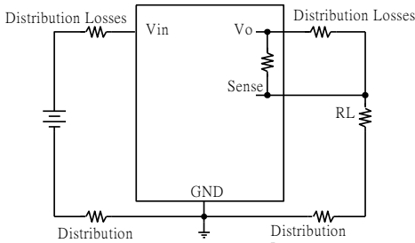
Figure 36: Effective circuit configuration for remote sense operation
