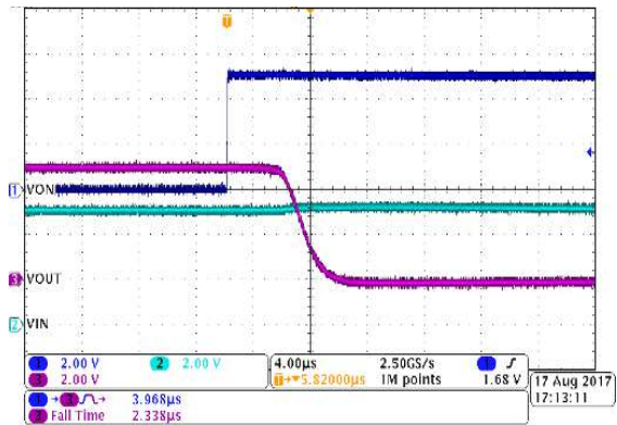
TPS22916CL V IN = 5 V C L = 0.1 μF R L = 10 Ω
