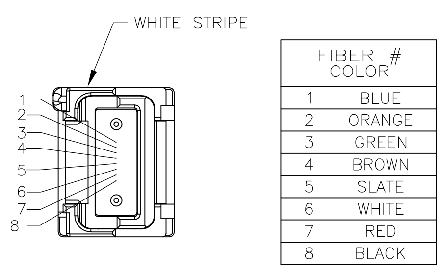
VIEW A-A LIGHTRAY MPX CONNECTOR FIBER PATH
