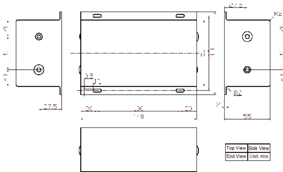
Figure 11. Dimensions for AHV12V30KVR7MAW
