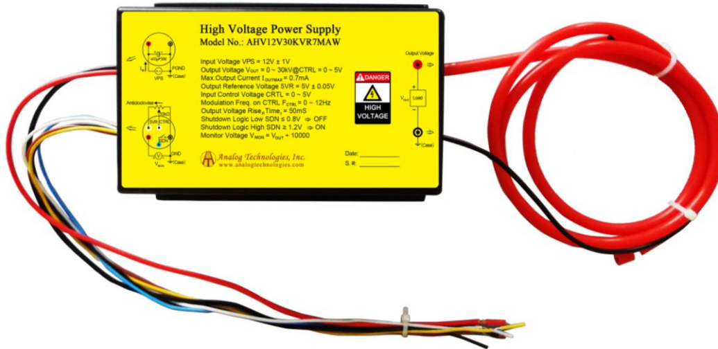
Figure 10. Leads of AHV12V30KVR7MAW
