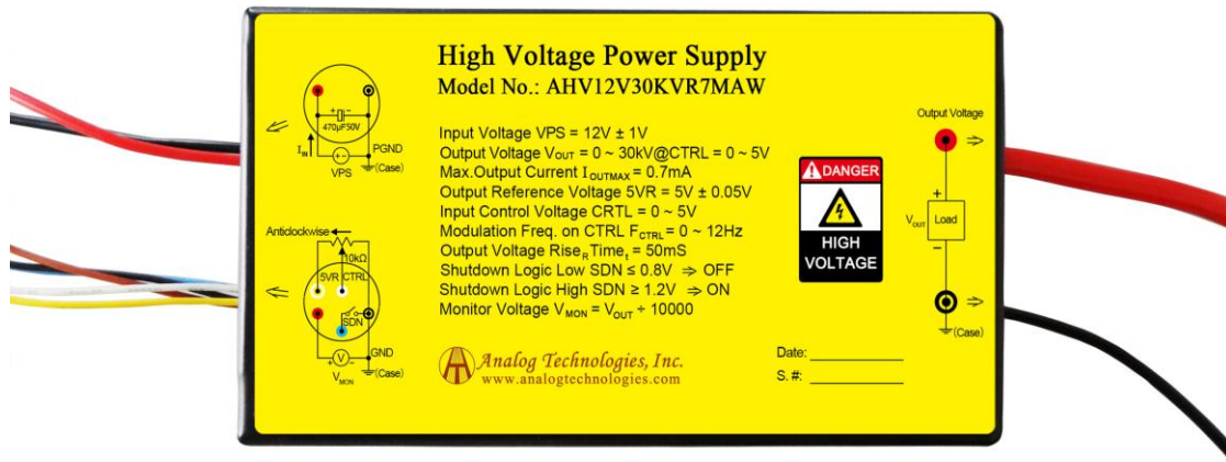
Figure 1. Physical Photo of AHV12V30KVR7MAW
