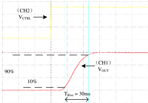
Figure 6. Rise Time
