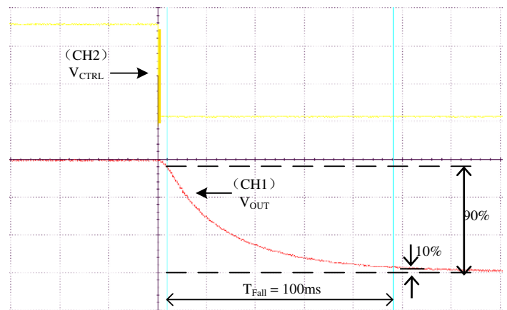
Figure 7. Fall Time
