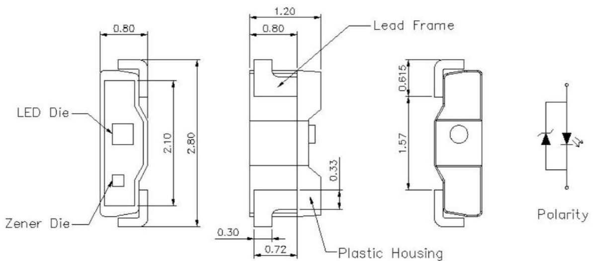
Figure 2. IN-P218AS Package Dimensions
