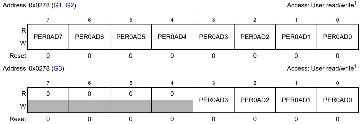
Figure 2-56. Port AD Pullup Enable Register (PER0AD)
