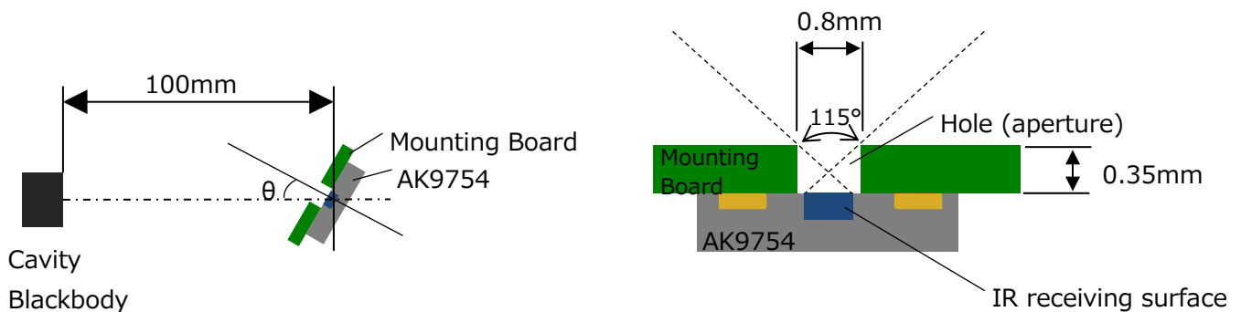
Figure 15.2. Measurement Environment
