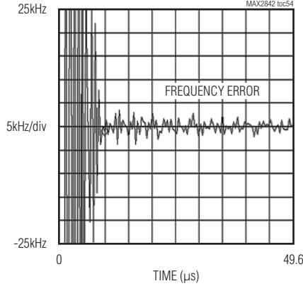
Rx-TO-Tx TURNAROUND FREQUENCY GLITCH SETTLING
