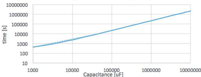
0V - 3V Charge Time vs Storage Capacitance
