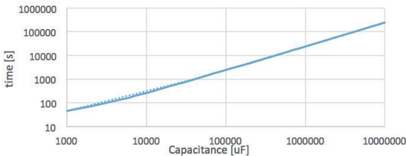
3V to 4.2V Charge Time vs Storage Capacitance
