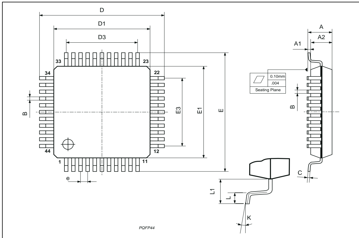
PQFP44 (10 x 10)
