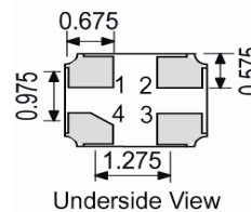
Underside View
