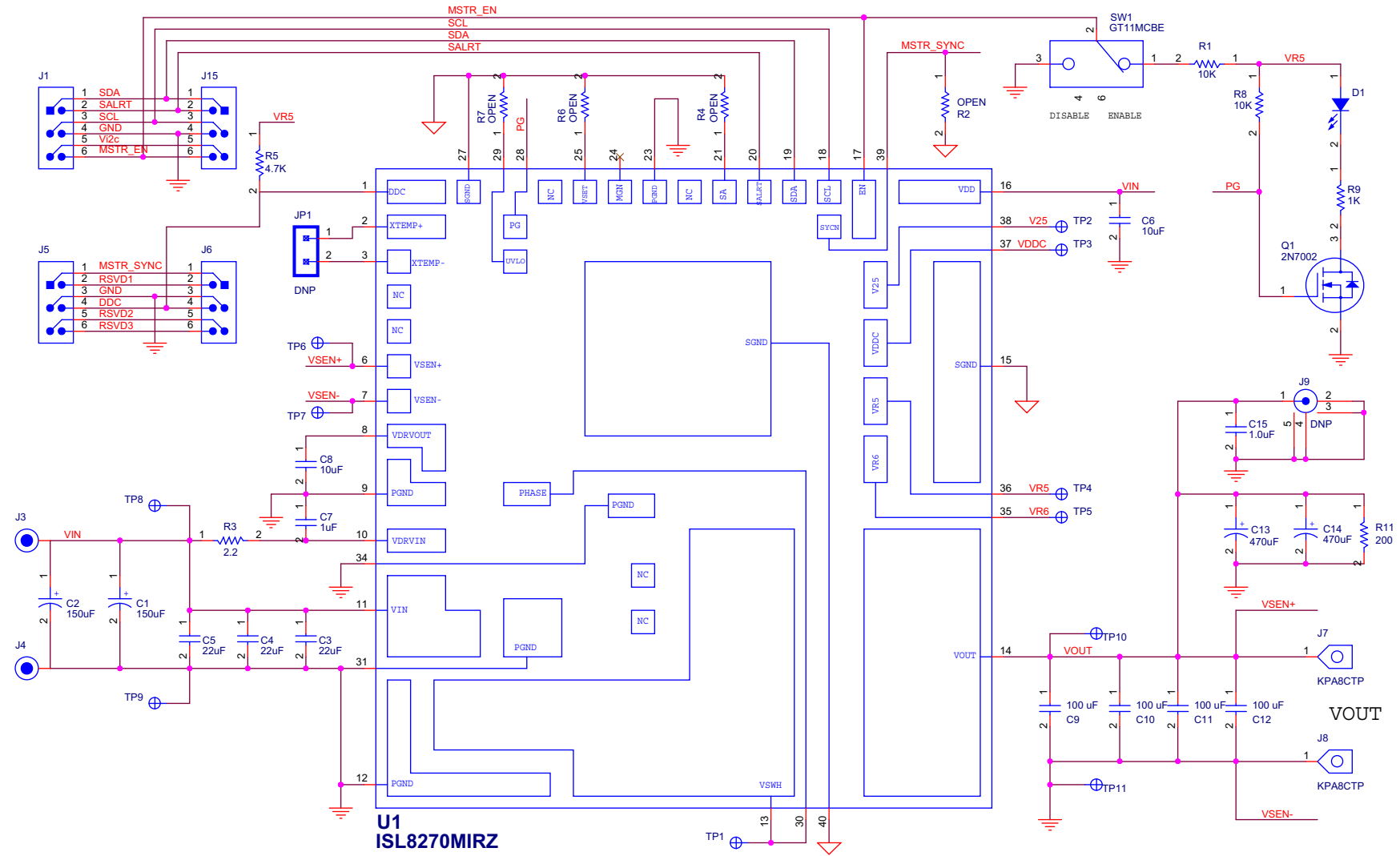
FIGURE 2. APPLICATION CIRCUIT
