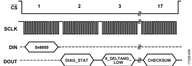
Figure 45. Burst Read Sequence with BURST_SEL = 1
