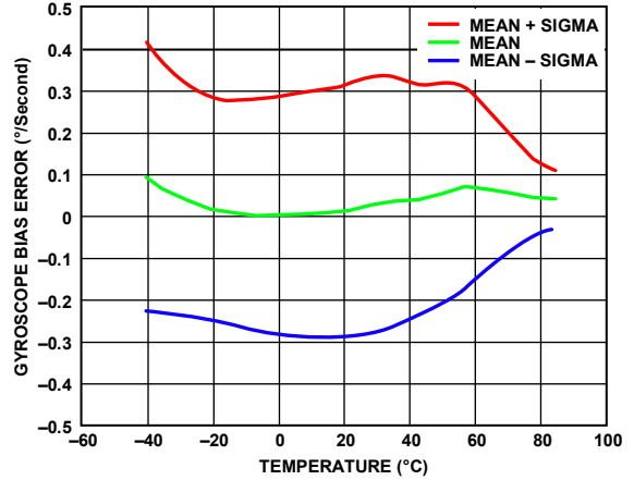
Figure 12. Gyroscope Bias Error vs. Temperature, ADIS16505-3, All Axes
