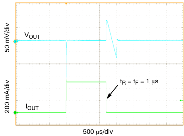
Figure 15. Load Transient Response, I_{OUT} = 1\text{ mA} to 500\text{ mA} , C_{OUT} = 2.2\ \mu\text{F}
