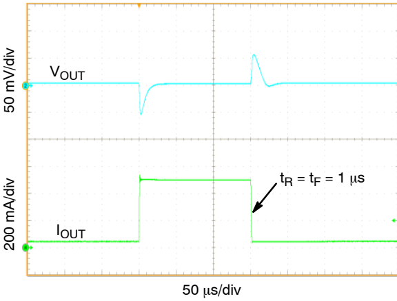
Figure 12. Load Transient Response, I_{OUT} = 50\text{ mA} to 500\text{ mA} , C_{OUT} = 10\ \mu\text{F}
