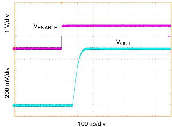
Figure 17. Enable Turn-on Response, I_{OUT} = 0\text{ mA} , C_{OUT} = 2.2\ \mu\text{F}
