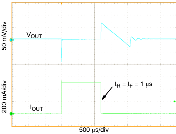
Figure 14. Load Transient Response, I_{OUT} = 1\text{ mA} to 500\text{ mA} , C_{OUT} = 10\ \mu\text{F}
