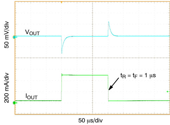
Figure 13. Load Transient Response, I_{OUT} = 50\text{ mA} to 500\text{ mA} , C_{OUT} = 2.2\ \mu\text{F}
