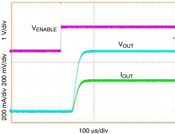
Figure 16. Enable Turn-on Response, Output Resistive Load 500\text{ mA} , C_{OUT} = 10\ \mu\text{F}
