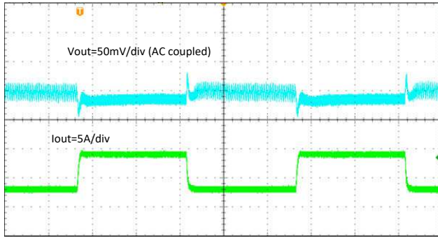
200us/div 0.1 A to 6 A Slew Rate = 2.5 A/μs
