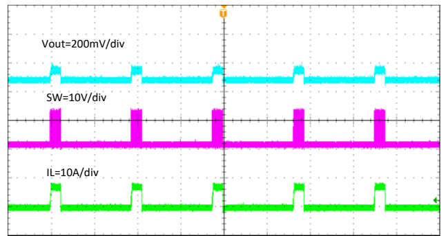
10ms/div
