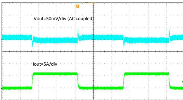
Figure 8-20. TPS566231 Transient Response
