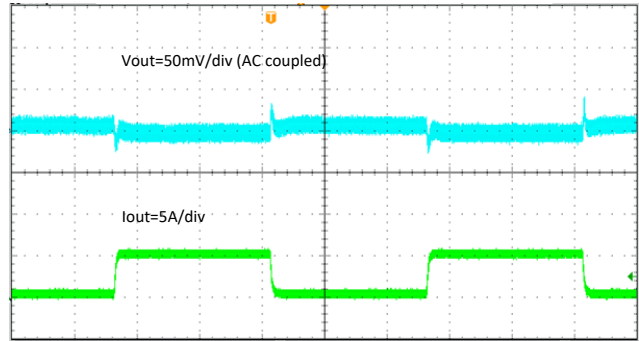
200us/div 0.6 A to 5.4 A Slew Rate = 2.5 A/μs
