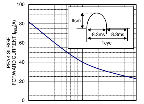
NUMBER OF CYCLES I_{FSM} -CYCLE CHARACTERISTICS
