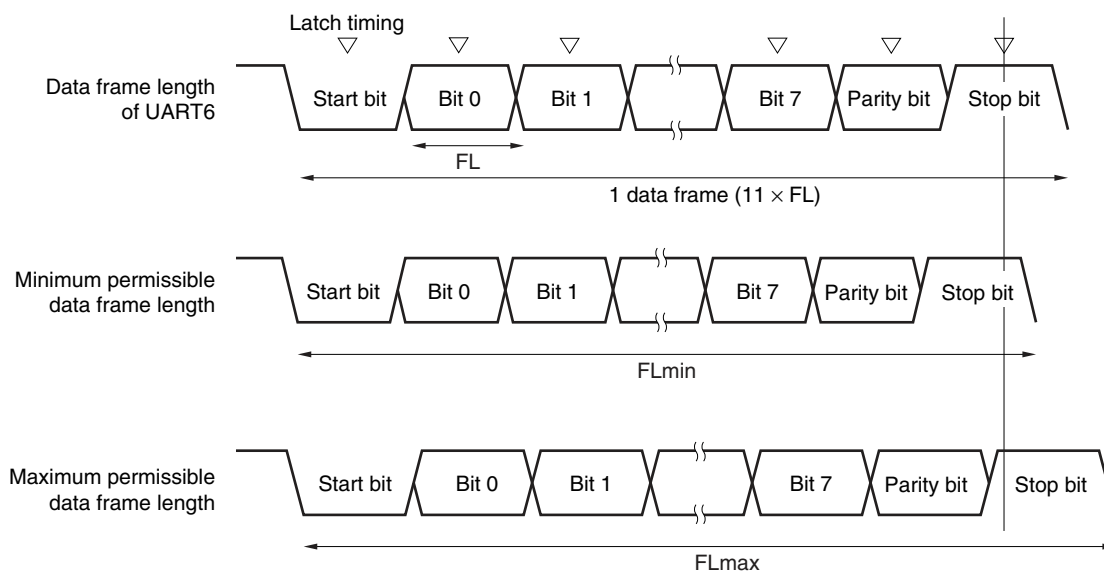
Figure 13-26. Permissible Baud Rate Range During Reception
