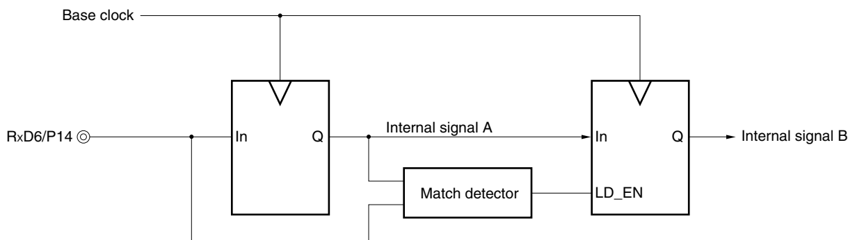
Figure 13-21. Noise Filter Circuit
