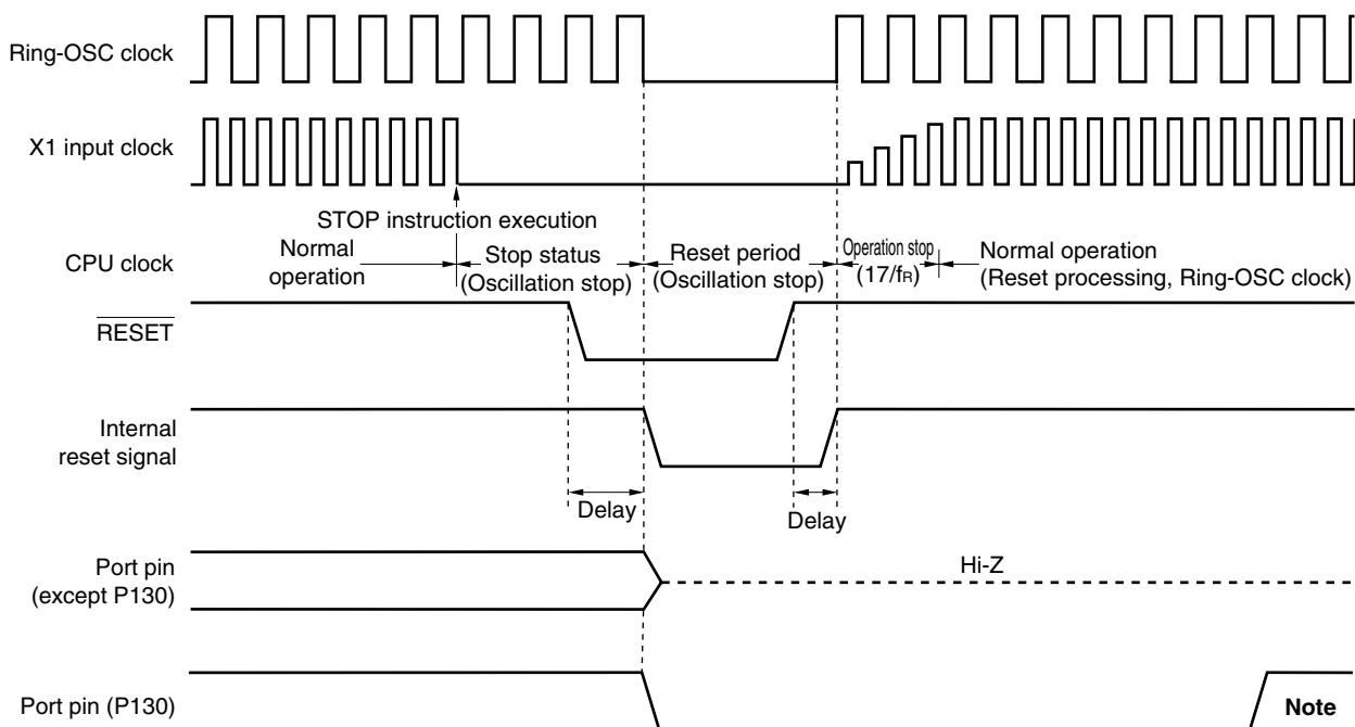
Figure 18-4. Timing of Reset in STOP Mode by \overline{\text{RESET}} Input
