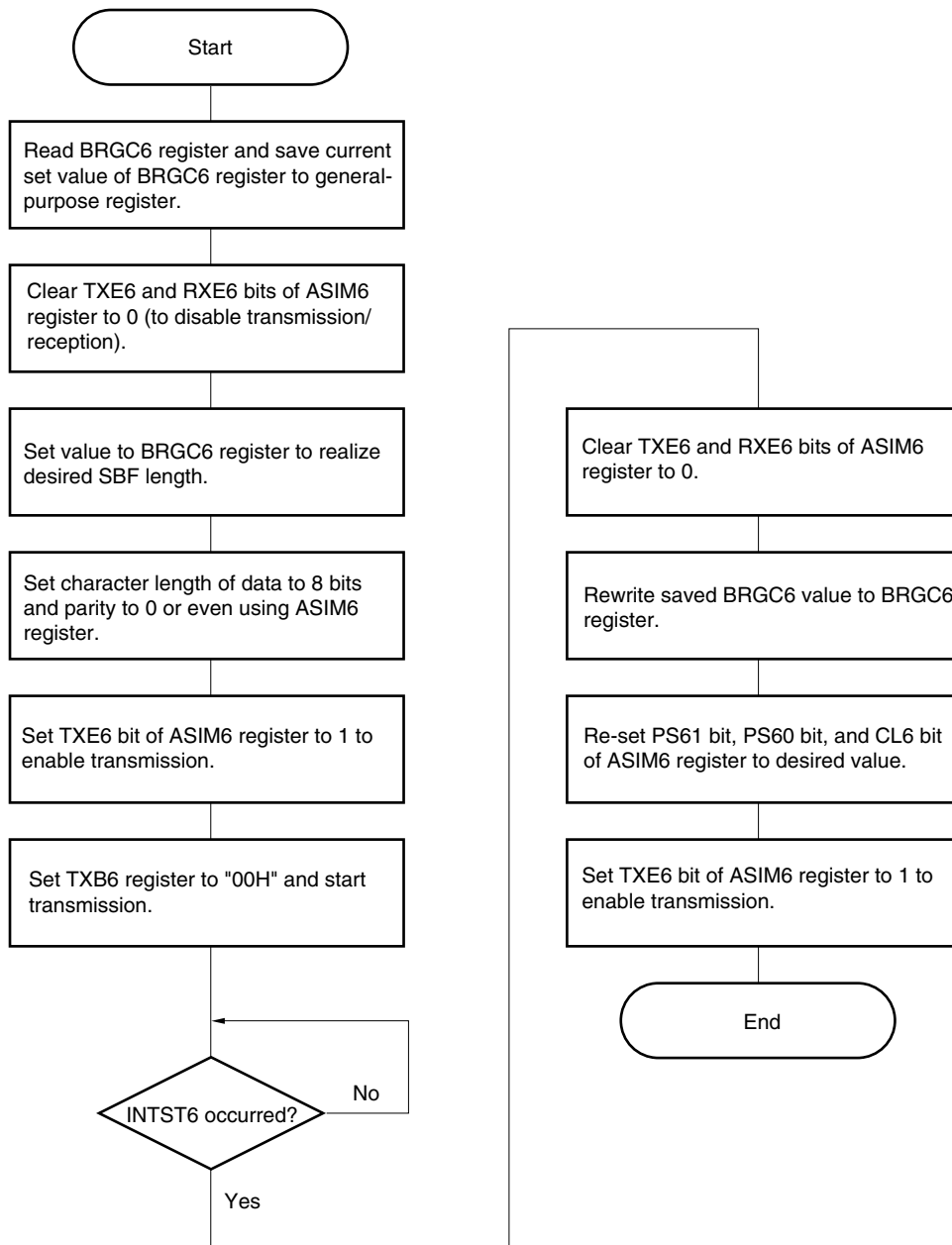
Figure 13-23. SBF Transmission
