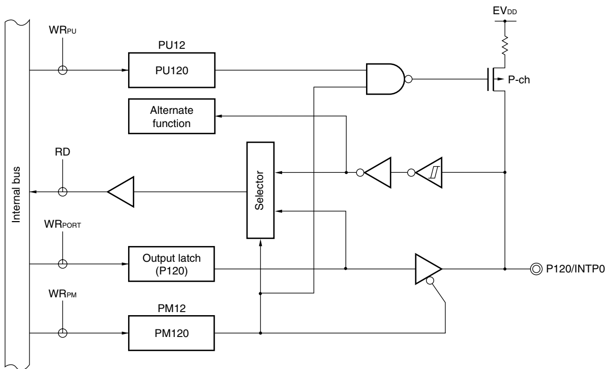
Figure 4-14. Block Diagram of P120
