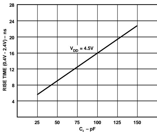
Figure 19. Typical Output Rise Time vs. Load Capacitance, C_L (at Maximum Ambient Operating Temperature)
