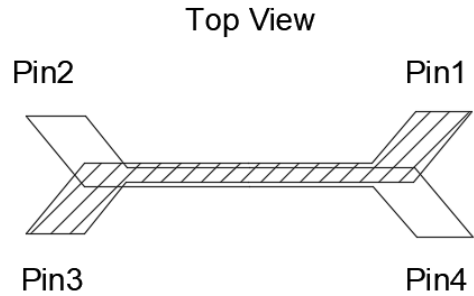
5dB Coupler Pin Configuration
