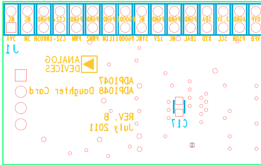
Figure 12 –Bottom Silkscreen
