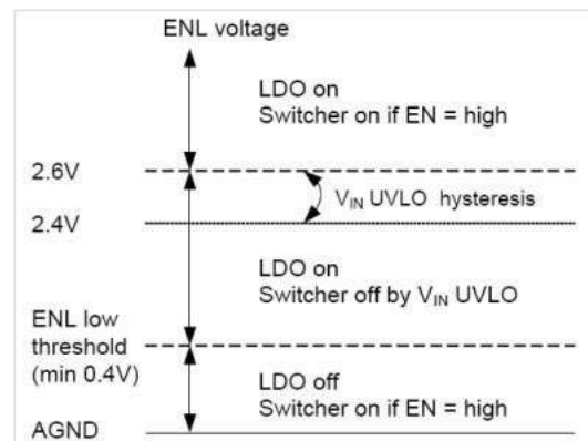
Fig. 11 - ENL Thresholds
