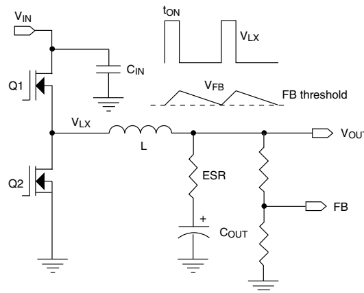
Fig. 1 - PWM Control Method, V_{OUT} Ripple
