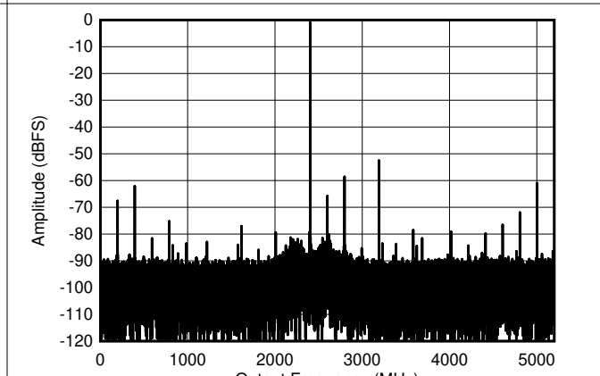
Figure 6-10. DES Mode: Single Tone FFT at 7997 MHz
