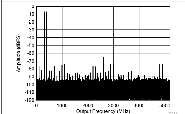
each tone at -7 dBFS, 100MHz Tone Spacing Figure 6-11. DES Mode: Two Tone FFT at 347 MHz
