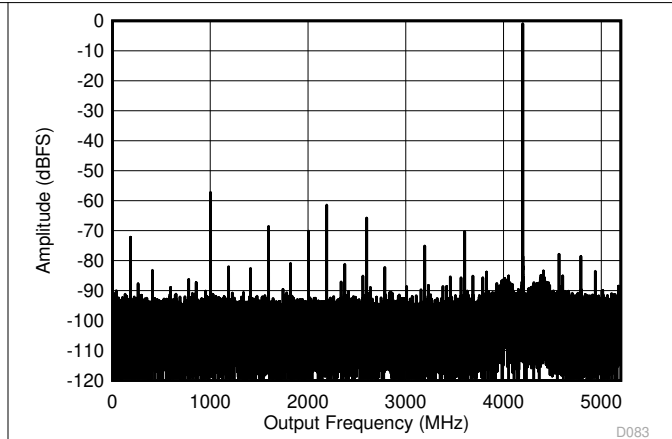
Figure 6-8. DES Mode: Single Tone FFT at 4197 MHz
