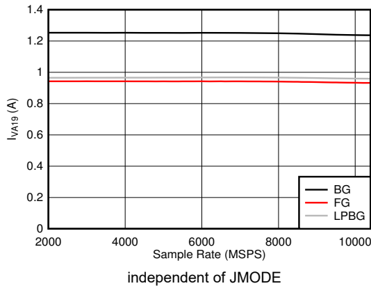
Figure 6-121. DES Mode: I_{VA19} vs Sample Rate
