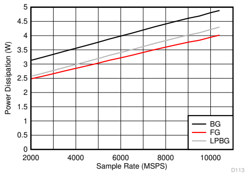
Figure 6-127. DES Mode: Power Dissipation vs Sample Rate
