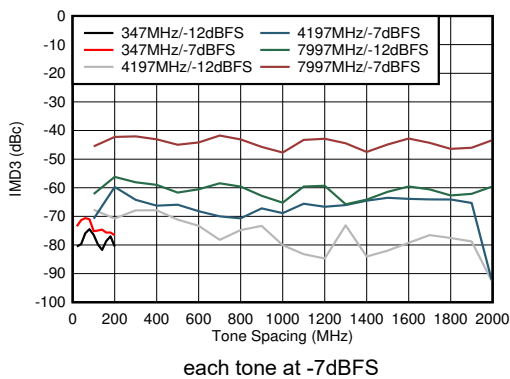
Figure 6-101. DES Mode: IMD3 vs Tone Spacing
