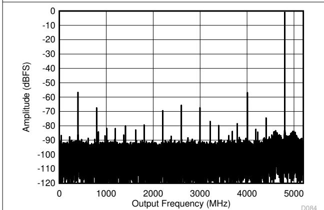
Figure 6-9. DES Mode: Single Tone FFT at 5597 MHz
