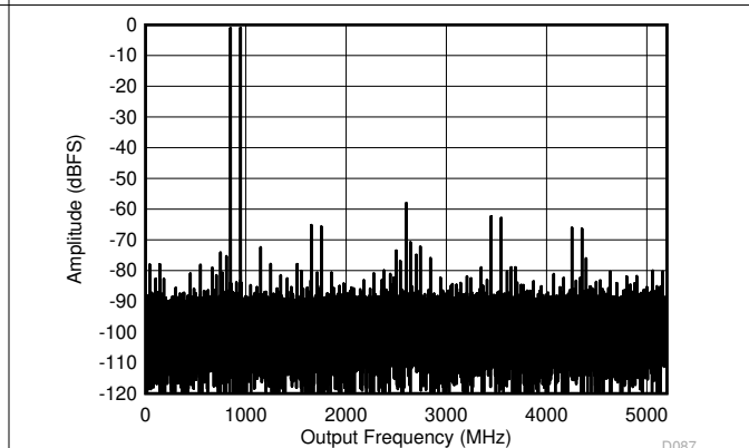
each tone at -7 dBFS, 100 MHz Tone Spacing Figure 6-12. DES Mode: Two Tone FFT at 897 MHz
