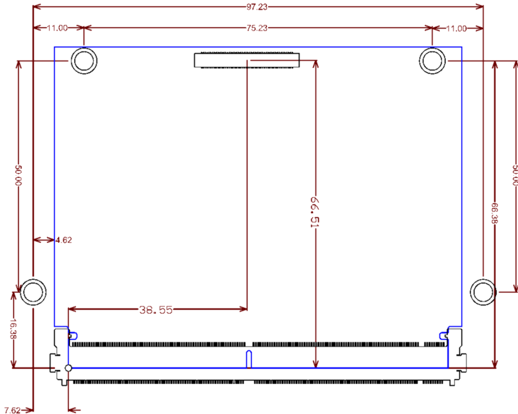
Figure 4 Recommended MitySOM-AM57F Carrier Card Outline with heat spreader mounting holes.
