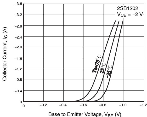
Figure 5. I_C - V_{BE}
