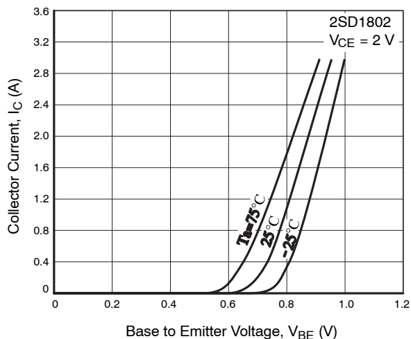
Figure 6. I_C - V_{BE}
