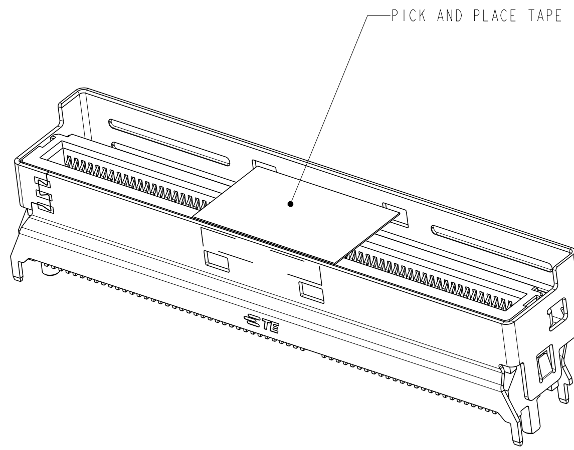
W/ PICK AND PLACE TAPE SCALE 4:1
