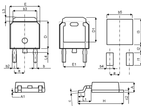
TO-252, (TO-252GE)
