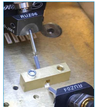
Top: Coplanar RF probe example Bottom: Example of test fixture
